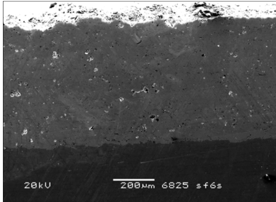
Cross section of thermal sprayed Stellite 6: Low porosity, no heat affected zone, minimal post treatment needed if necessary
