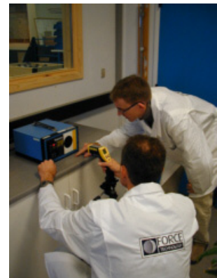
Calibration of pyrometer against black-body
